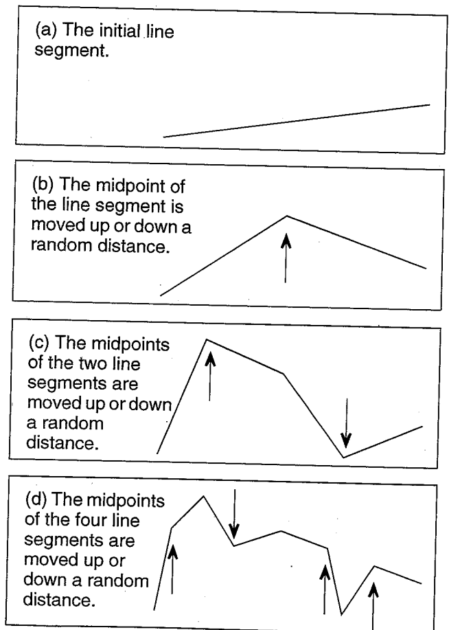
FIGURE 8.3 The First Few Steps in Generating a Random Fractal
